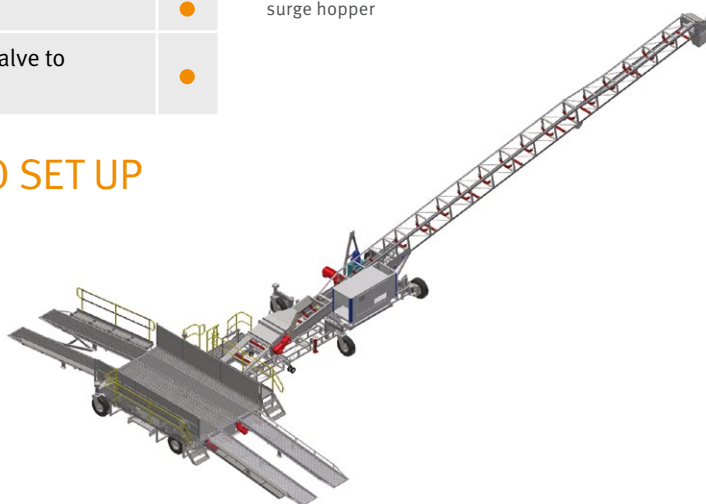
Out loading via BunkerStacker 3000 fitted with surge hopper
