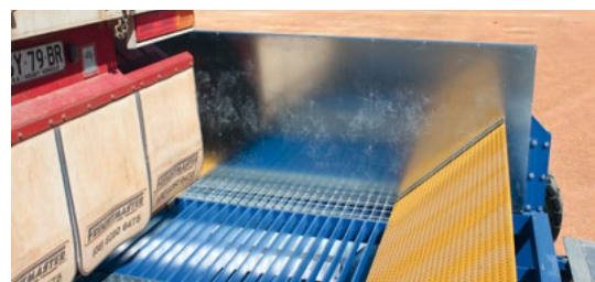
Raised hungry boards on Drive Over Hopper
